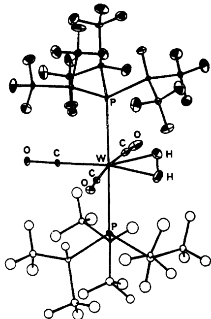
Figure 1. Structure of W(CO)_3(PPR^i_3)_2(H_2) (neutron, 30 K). (Disorder is present in C-H positions of lower phosphine.)
